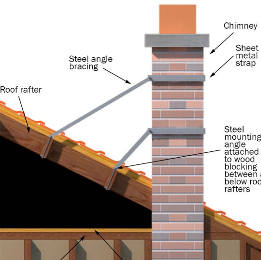
Figure C. Bracing masonry chimneys.
