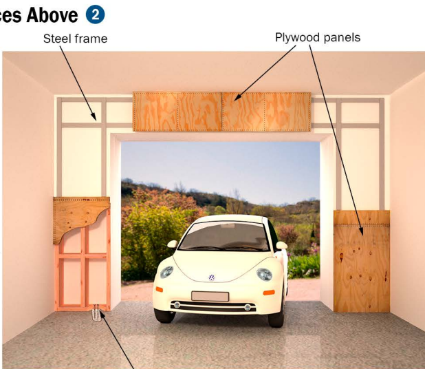
Figure B. Strengthening garage walls below living space.
